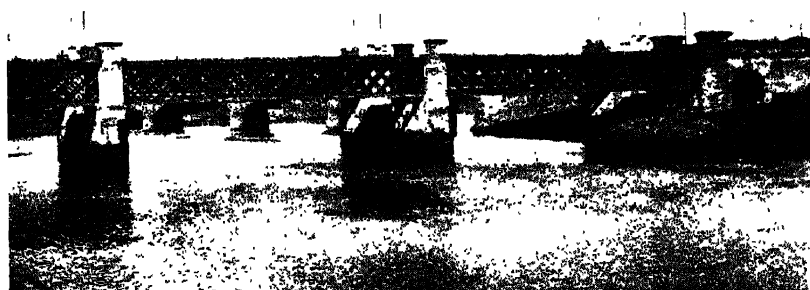
Fig. 7.—Railway Bridge at Stirling. A TYPICAL UTILITARIAN STRUCTURE; NOTE THE PIERS OF THE ROAD BRIDGES IN THE BACKGROUND. [THESE THREE PHOTOGRAPHS PROVIDE AN INTERESTING COMPARISON OF DIFFERENT PERIODS OF BRIDGE CONSTRUCTION. THE BRIDGES SPAN THE SAME RIVER WITHIN A DISTANCE OF 400 FT.]
